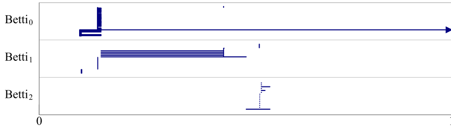
Figure 4: Spiral on a torus
